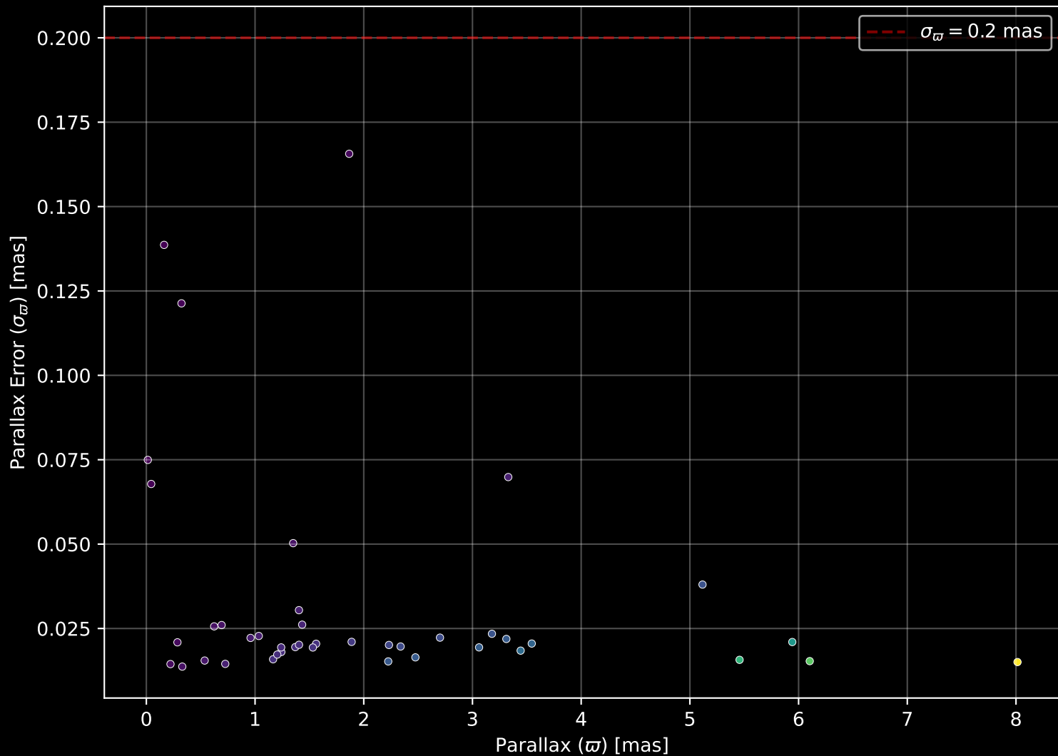
APOGEE DR17 Field: [ANDR1] Parallax Quality (n= 42)
