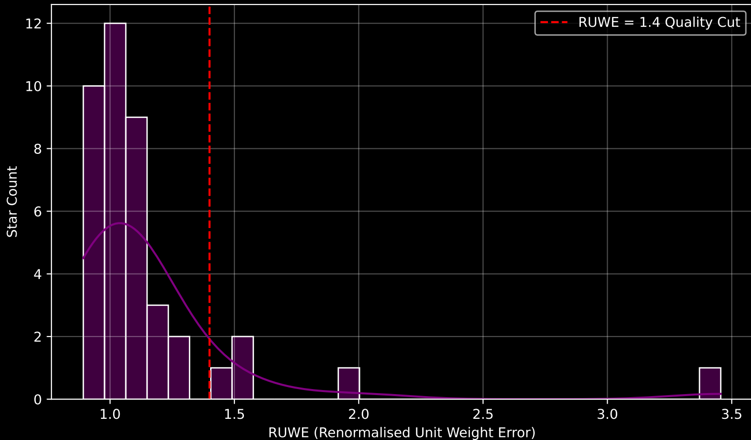
GAPOGEE DR17 Field [ANDR1] RUWE Distribution (n= 41)
