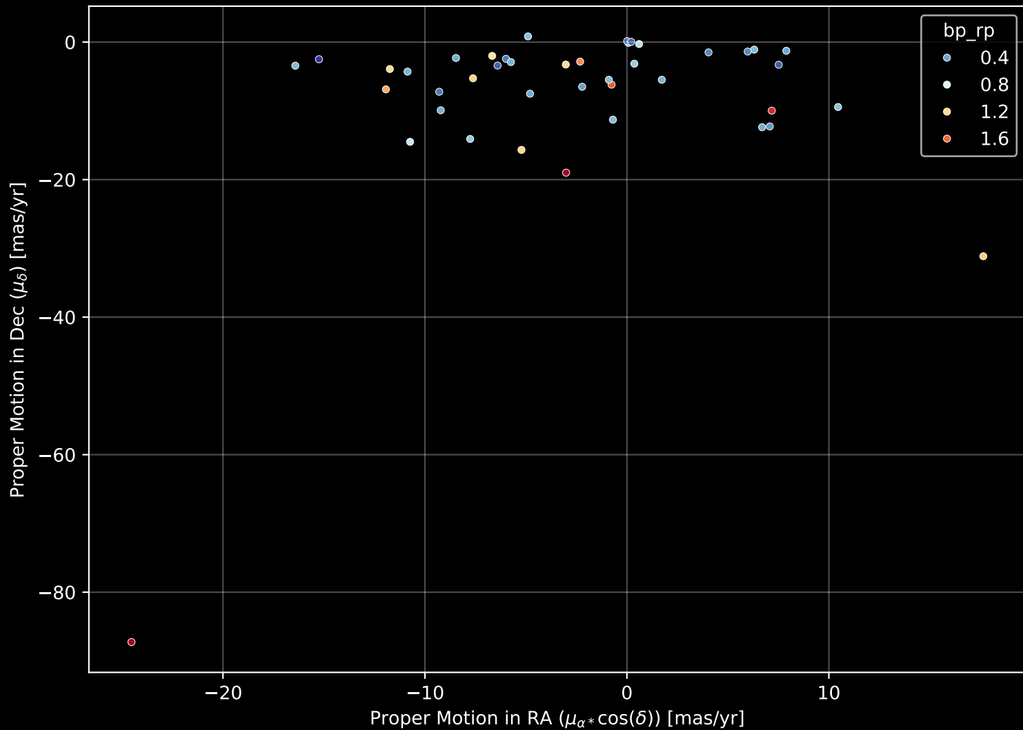
APOGEE DR17 Field: [ANDR1] Proper Motion Diagram (n= 42)
