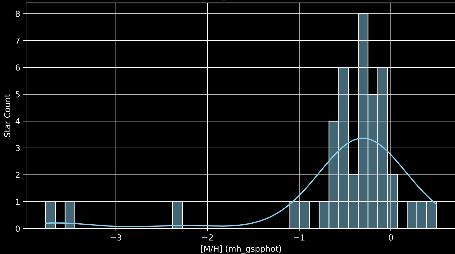
APOGEE DR17 Field: [ANDR1 [M/H] (mh_gspphot) (n= 42)
