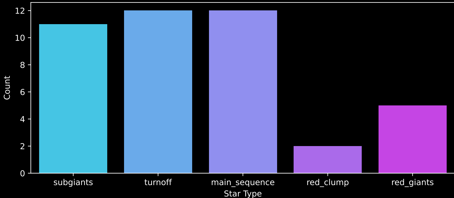
APOGEE DR17 Field: [ANDR1] Count plot of Star Type
