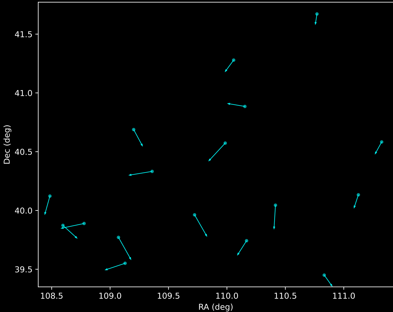
APOGEE DR17 Noise Stream Proper Motion Vectors (n=17)
